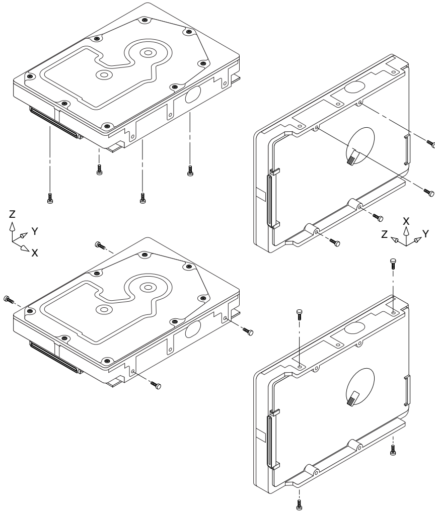
Figure 11. Recommended mounting
