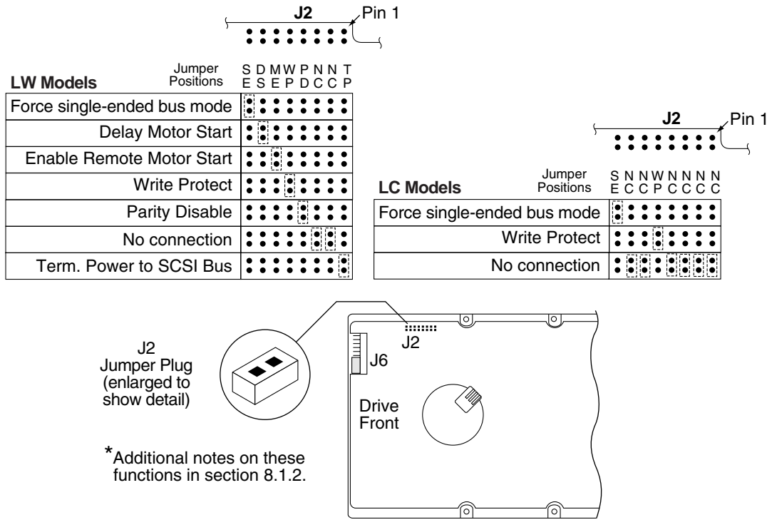
Figure 16. J2 option select header (on LW models only)
