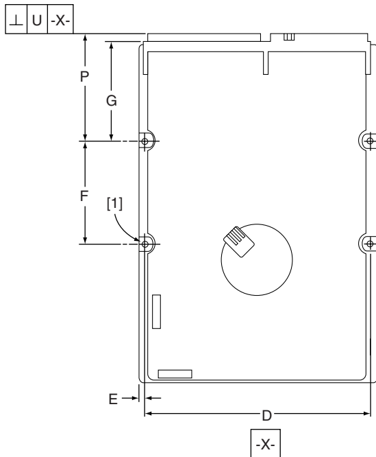
Figure 12. LW mounting configuration dimensions
