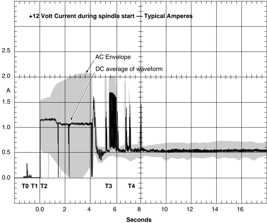
Figure 4. Typical ST318452 and ST318432 drive +12 V current profile
