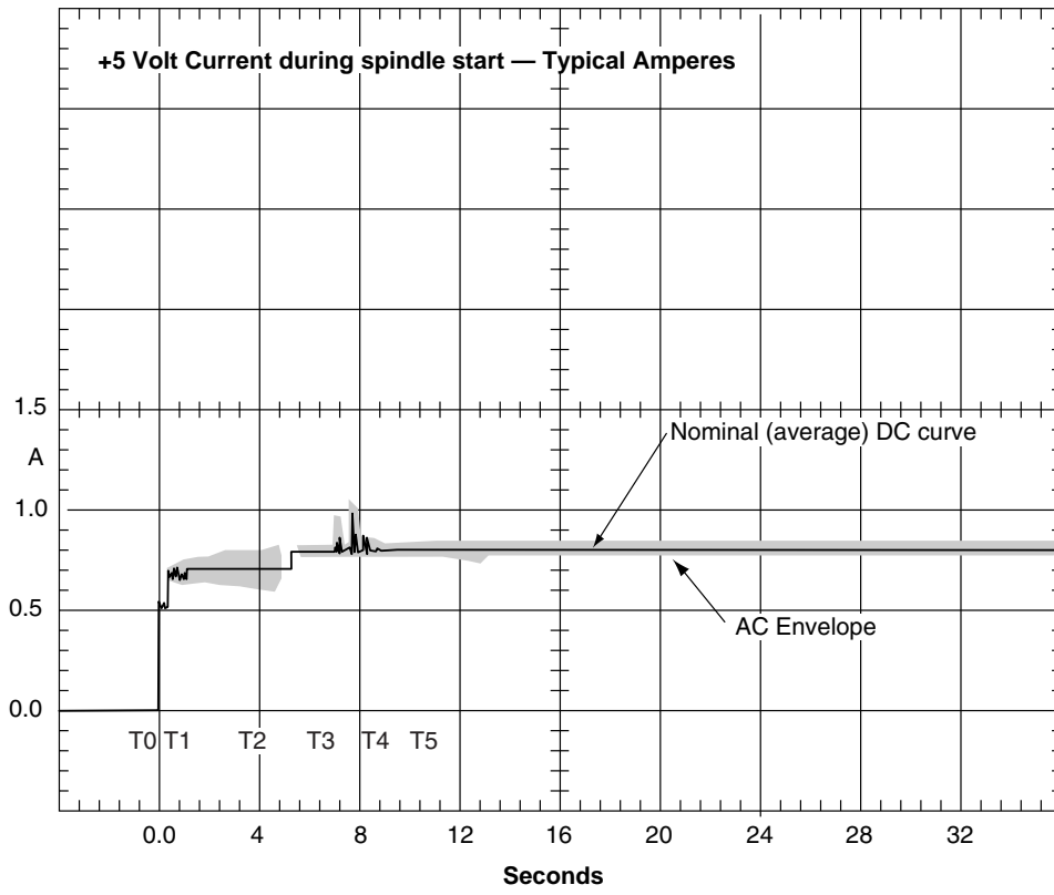
Figure 5. Typical ST318452 and ST318432 drive +5 V current profile
