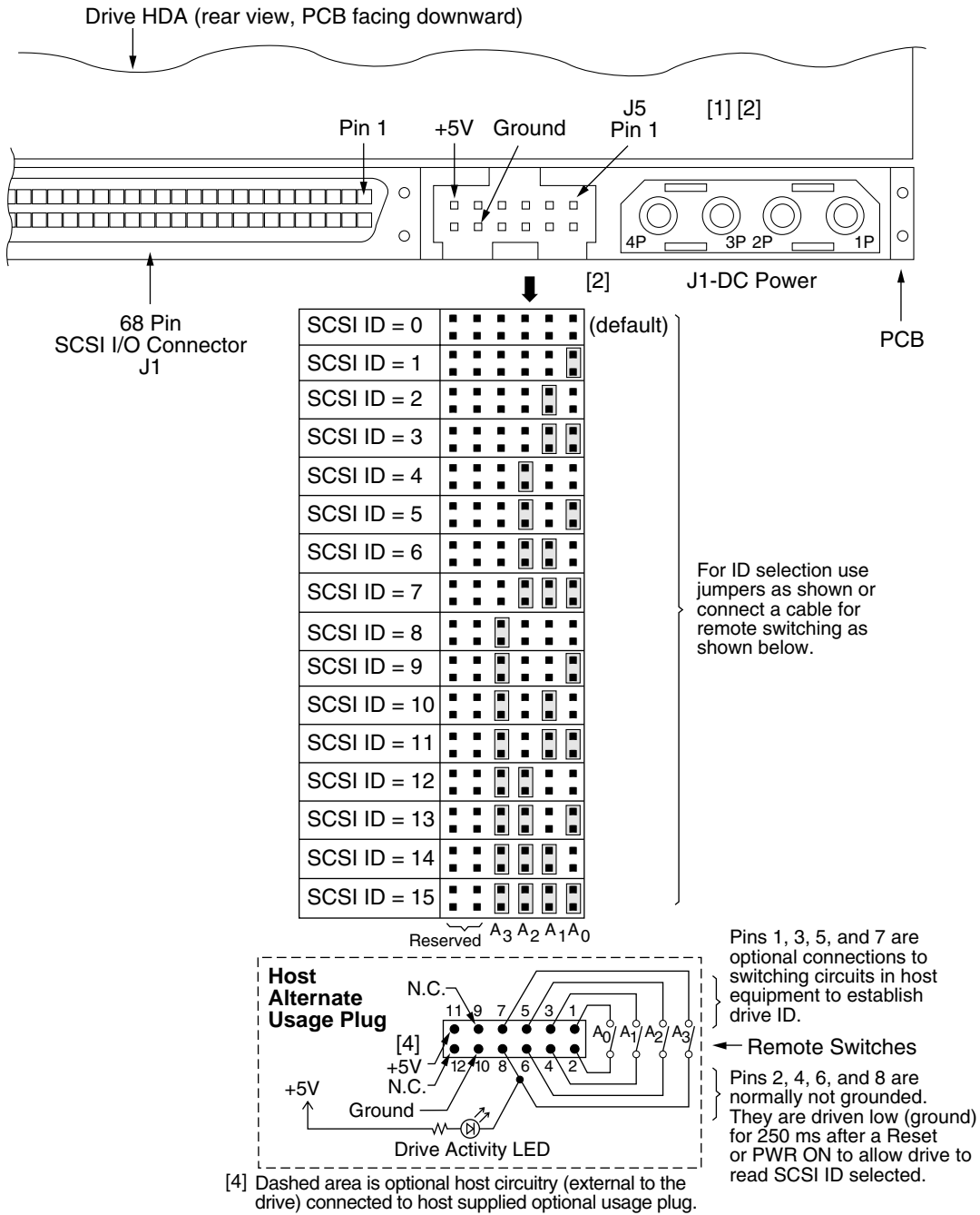
Figure 15. J5 jumper header (on LW models only)
