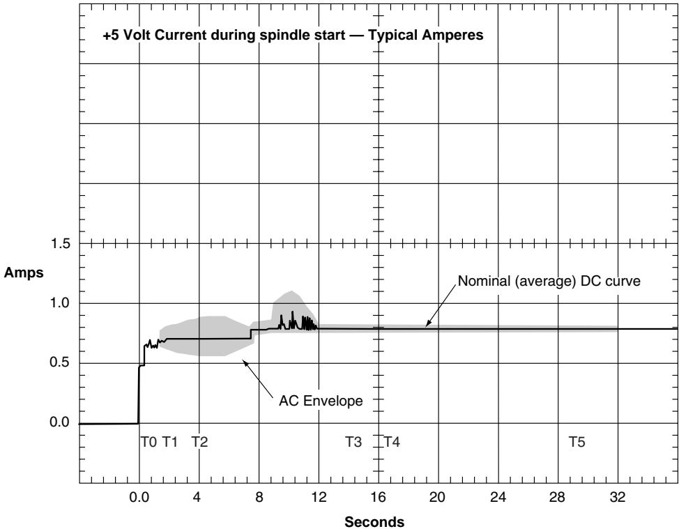
Figure 3. Typical ST336752 and ST336732 drive +5 V current profile
