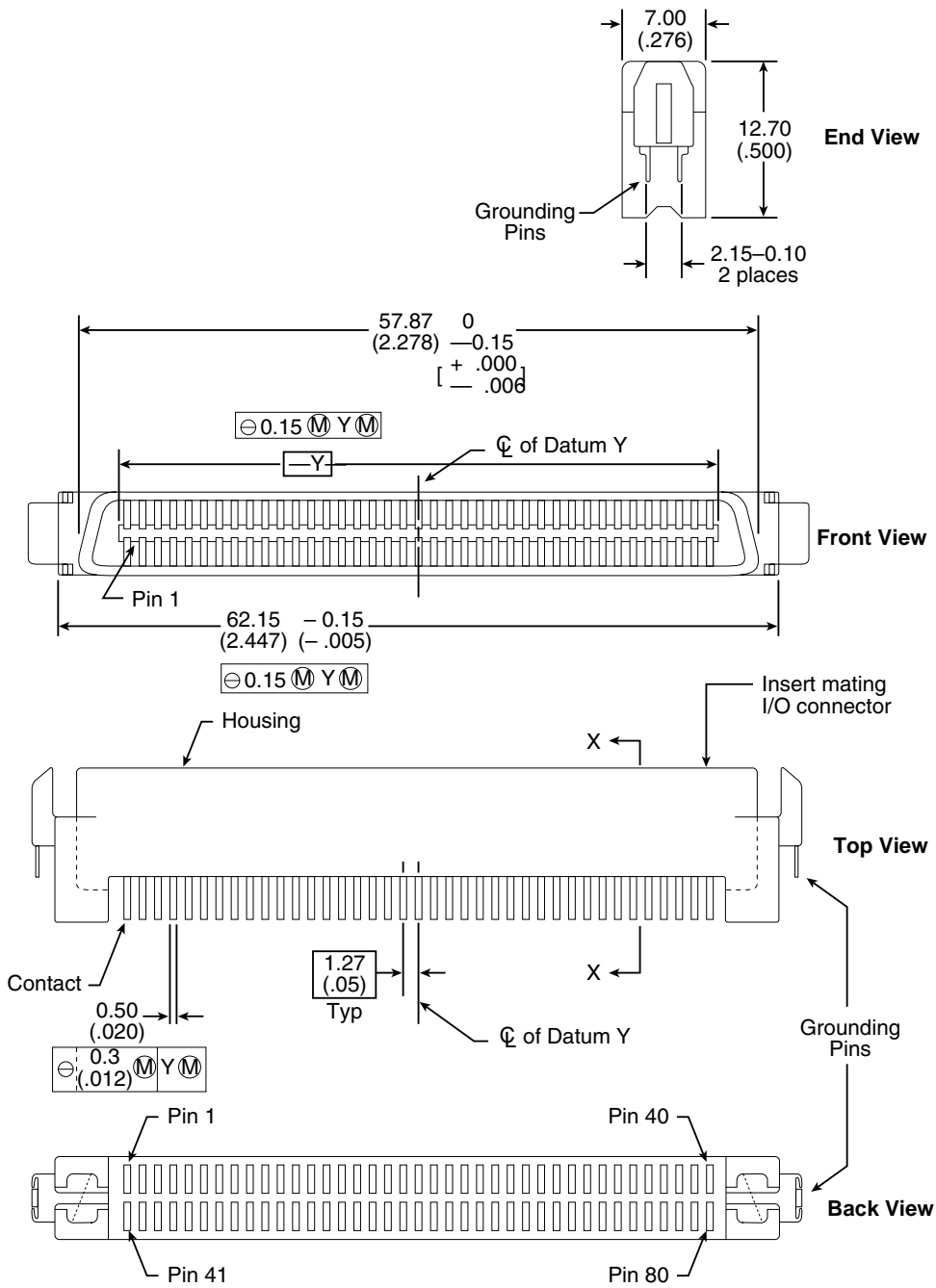
Figure 22. Nonshielded 80 pin SCSI "SCA-2" connector, used on LC drives
