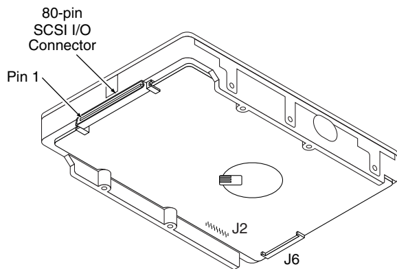
Figure 19. LC model drive physical interface (80-pin J1 SCSI I/O connector)
