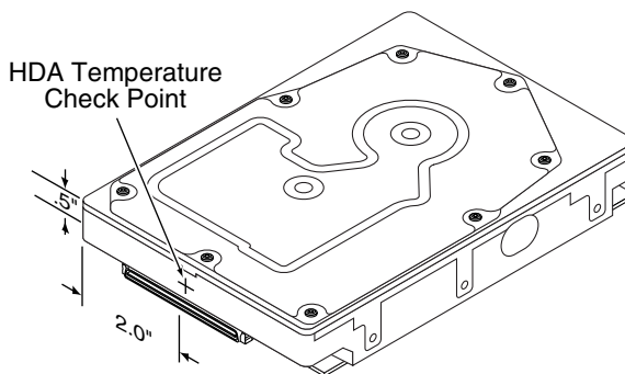
Figure 10. Locations of the HDA temperature check point
