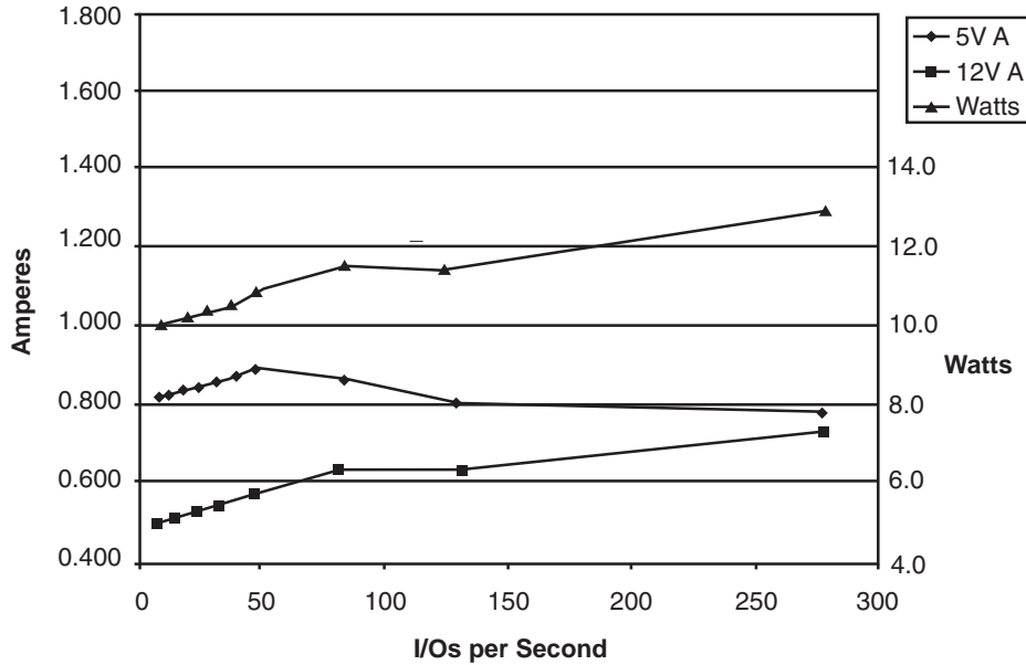
Figure 8. ST318452 and ST318432 DC current and power vs. IOPS (SE)
