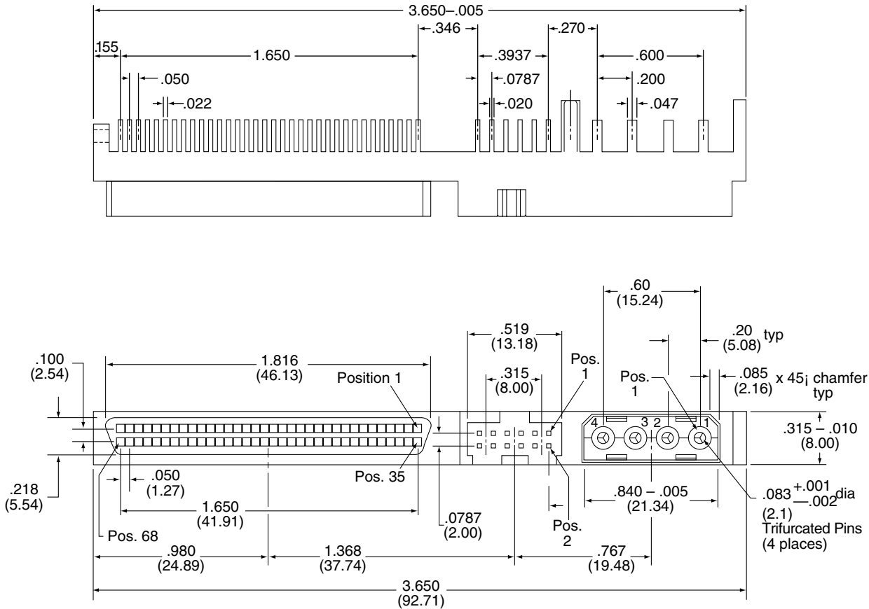
Figure 21. Nonshielded 68 pin SCSI device connector used on LW drives
