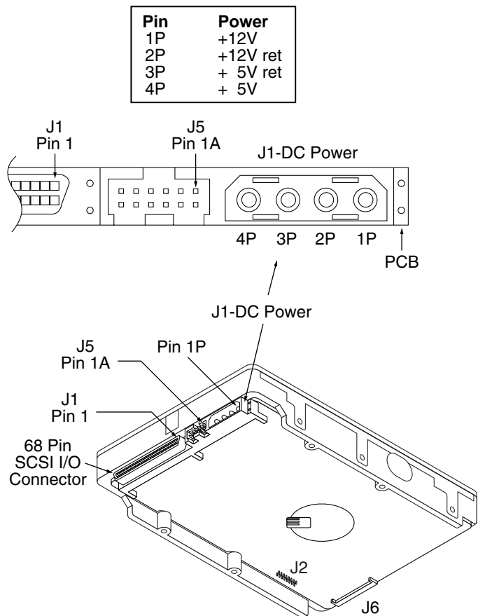
Figure 18. LW model drive physical interface (68-pin J1 SCSI I/O connector)
