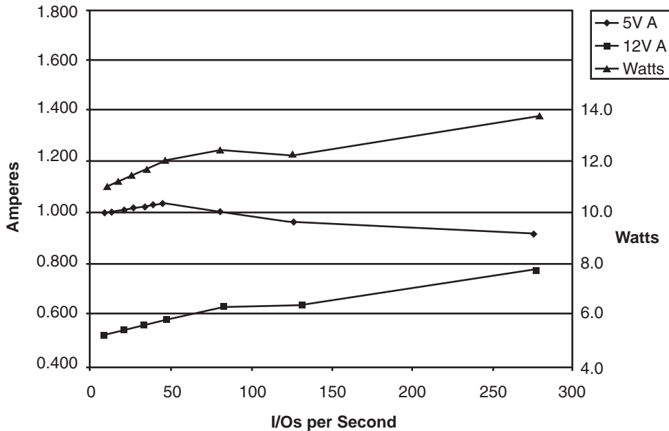
Figure 9. ST318452 and ST318432 DC current and power vs. IOPS (LVD)
