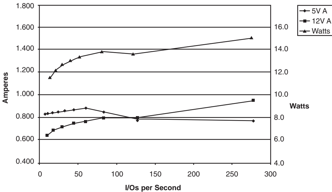
Figure 6. ST336752 and ST336732 DC current and power vs. IOPS (SE)
