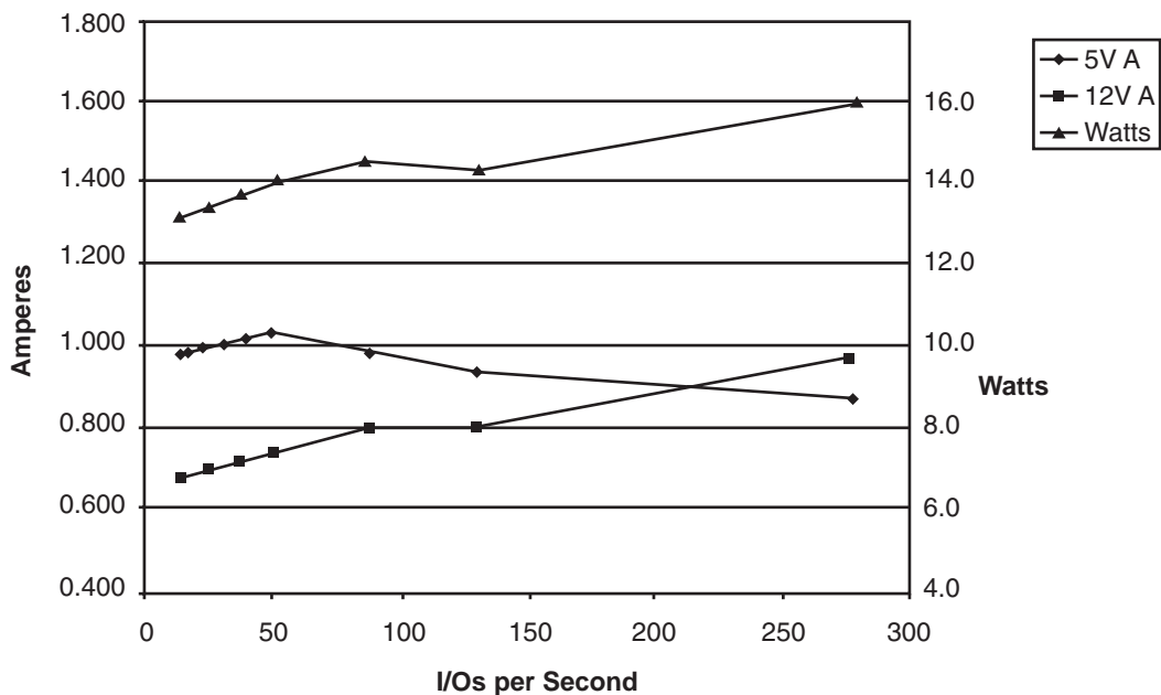
Figure 7. ST336752 and ST336732 DC current and power vs. IOPS (LVD)
